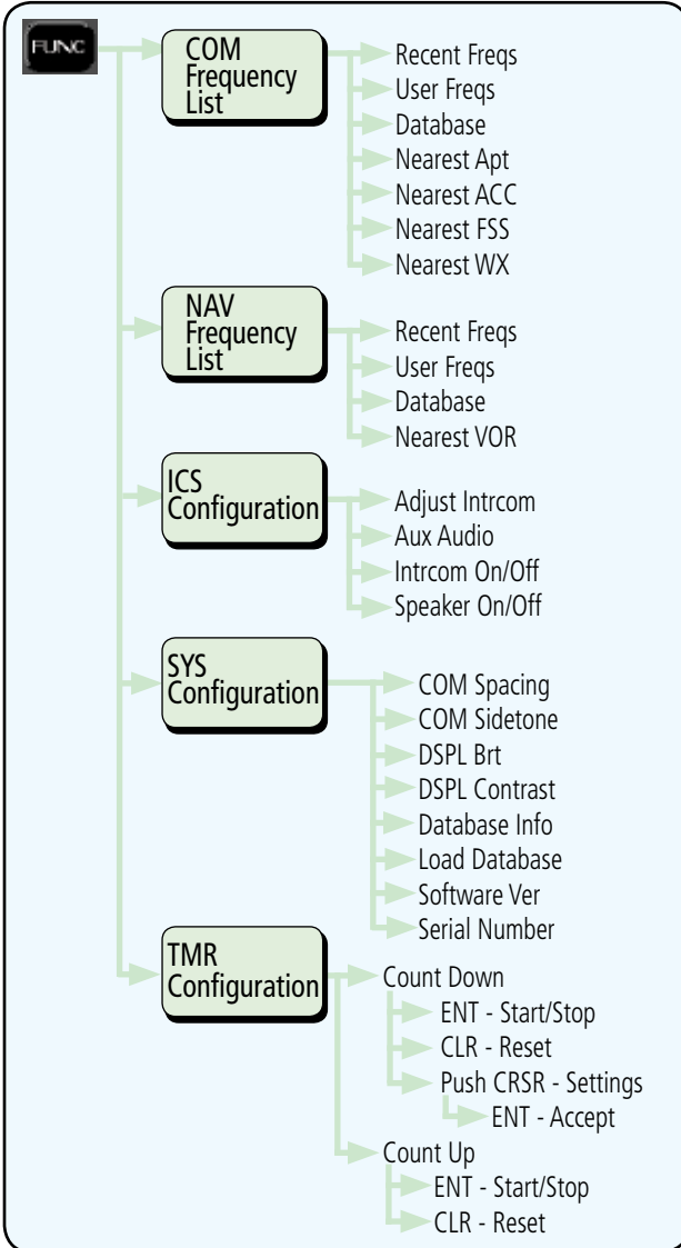
Functions Diagram
