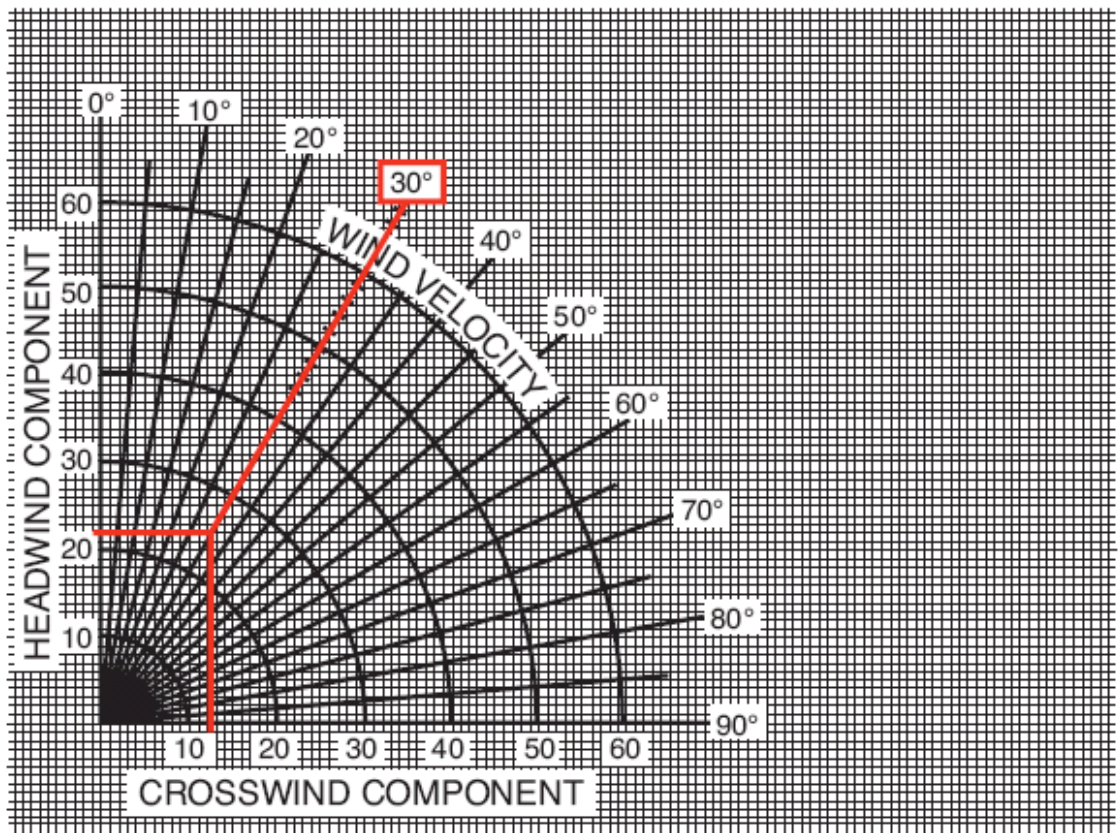
Figure 9-32. Crosswind component chart.
